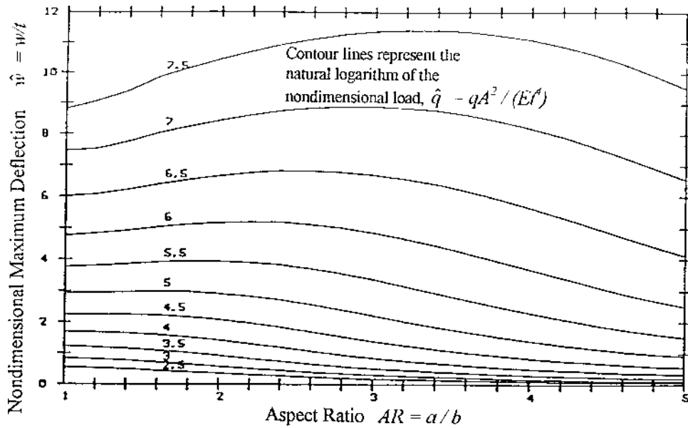
FIG. X1.1 Deflection Chart
