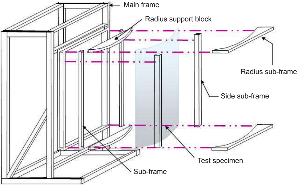
Figure 11 – Bent glass impact test frame (Exploded view)
