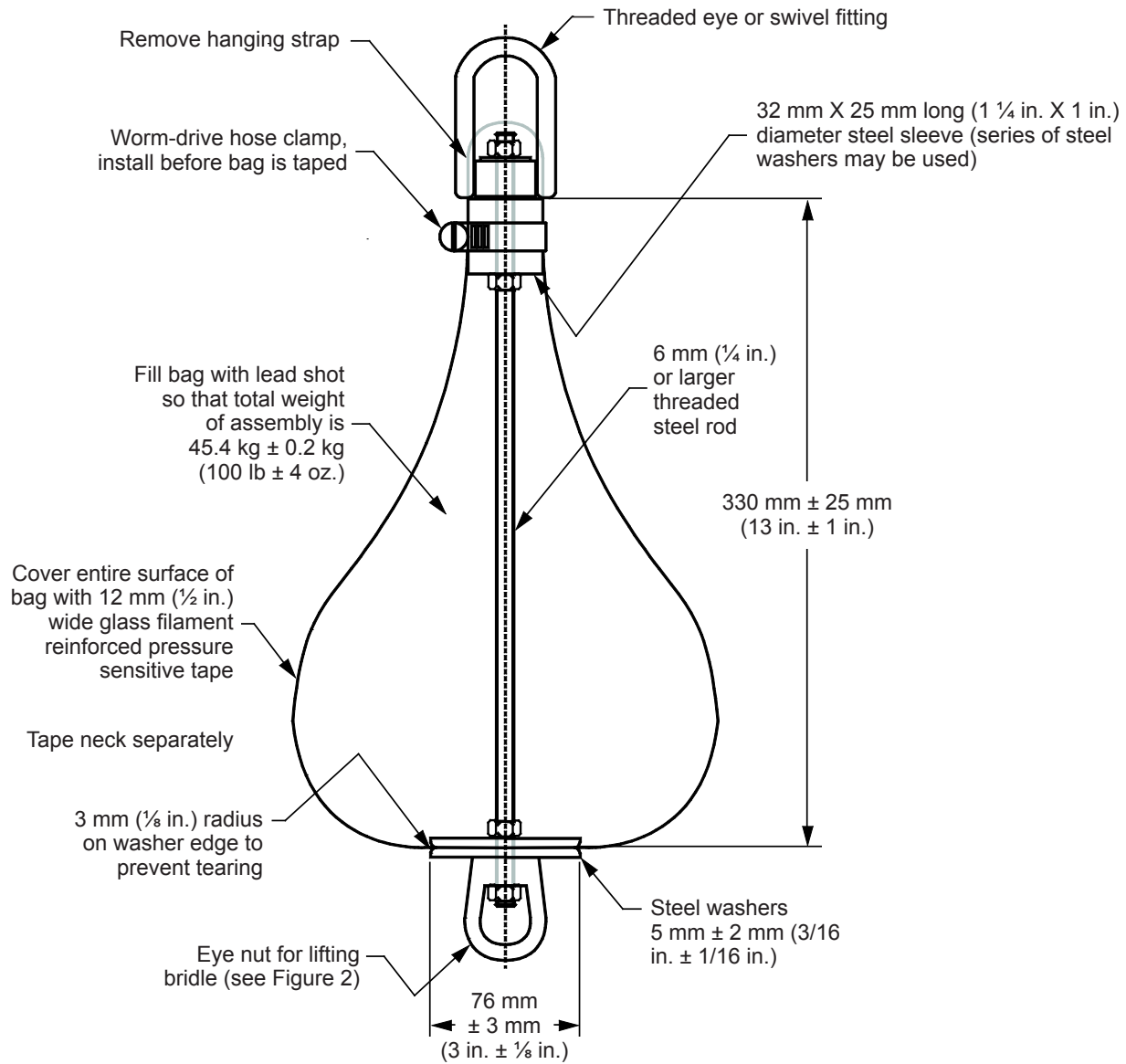
Figure 13 – Impactor
