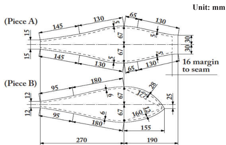
Figure 2 – Impactor bag
